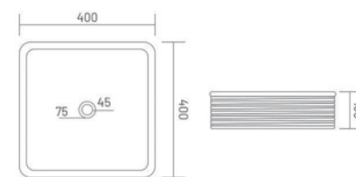
LUXORA Table Top Basin L 400 W 400 H 150
